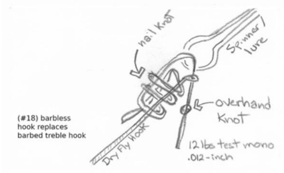
Drawings to help demonstrate the method for attaching the spinner and hook using monofilament fishing line.
